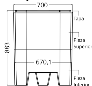
Alzado Principal
